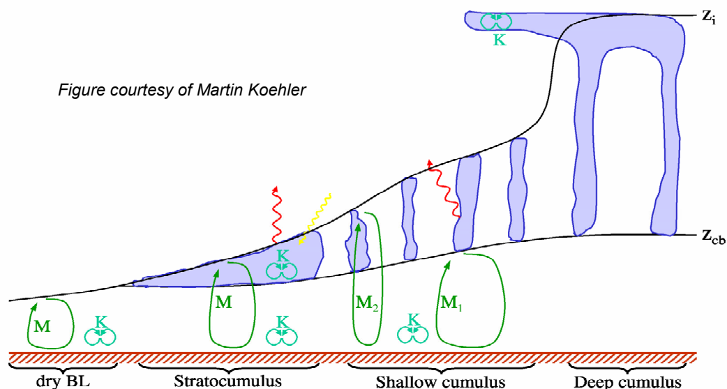
Figure 1: Schematics of the principle of the EDMF scheme. Note that the mass flux part, that is representing the thermals, is active in both the clear and the cloudy boundary layer. Therefore a trigger function for moist convection is not necessary anymore.
