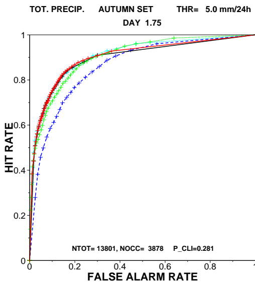
Figure 4 a, b) The figure shows the ROC-diagrams for two threshold values of total precipitation rates, looking at the cases in the autumn set at forecast time +42 hours. The threshold values are a) 5 mm/24h and b) 25mm/24h.
