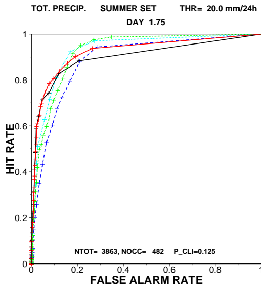
Figure 7 a, b) The figure shows the ROC-diagram for two different threshold values of total precipitation rates looking at the cases in the summer set at forecast time +42 hours. The threshold values are a) 20 mm/24h and b) 30mm/24h.
