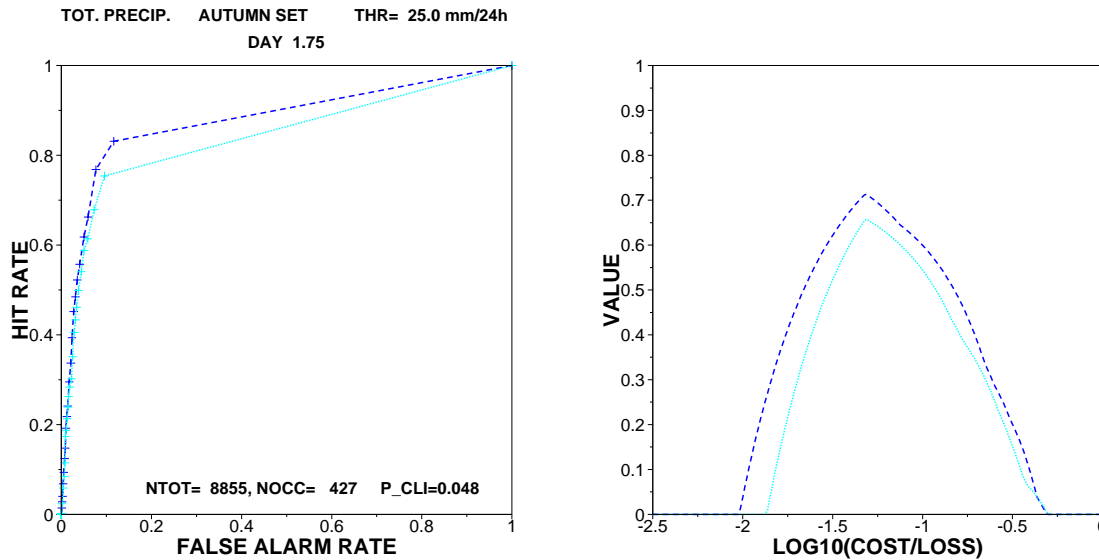
Figure 2. The ROC-diagram (to the left) and cost/loss-diagram (to the right) for LAMEPS (blue) and LAMEPS_SV (cyan) computed for the verification area and the 9 cases in the first set (autumn1 in table 1) at forecast time +42 hours. The threshold value is 25 mm/24 hours. NTOT is the total possible number the event could occur (the number of points in the target area multiplied by the number of cases) while NOCC is the number of times the event occurred in the sample. P_CLI is the total precipitation frequency in the experiment period (the sample climatology).
