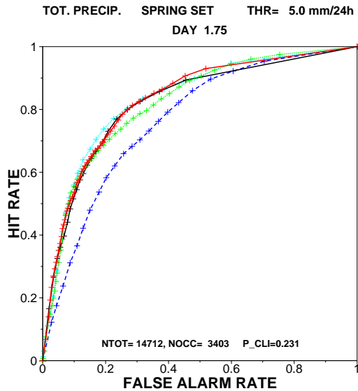
Figure 6 a, b) The figure shows the ROC-diagram for two different threshold values of total precipitation rates looking at the cases in the spring set at forecast time +42 hours. The threshold values are a) 5 mm/24h and b) 15 mm/24h.
