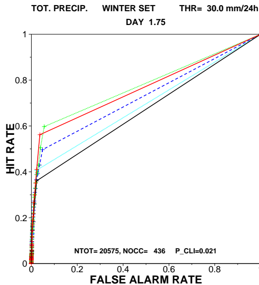
Figure 5 a, b) The figure shows the ROC-diagram for two different threshold values of total precipitation rates looking at the cases in the winter set at forecast time +42 hours. The threshold values are a) 10 mm/24h, b) 30mm/24h.
