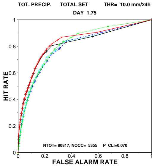
Figure 3 a, b) The figure shows the ROC-diagrams for two different threshold values of total precipitation rates where all the experiment sets are included. The threshold values are a) 10mm/24h and b) 25 mm/24h. The different curves are EPS (red), EPS20 (black), TEPS (light blue), LAMEPS (blue) and CLAMEPS (green).
