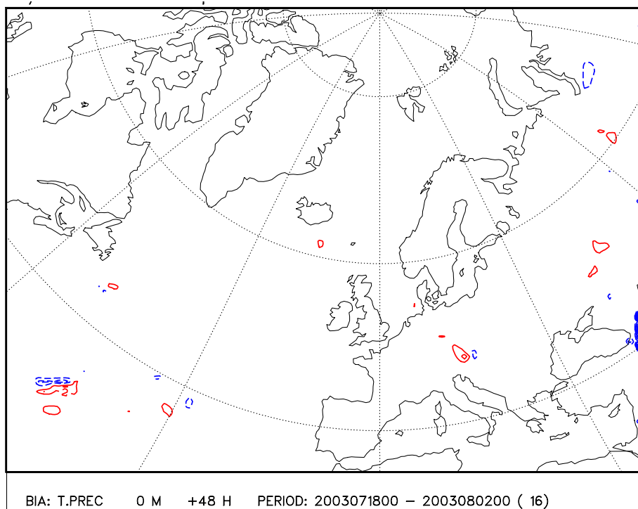
Figure 7: Systematic difference in 48 h accumulated total precipitation between REL and REF forecasts (REL-REF) for the period 16-31 July 2003. Contour interval: 2 mm. The zero isoline not plotted, negative values indicated with dashed lines.
