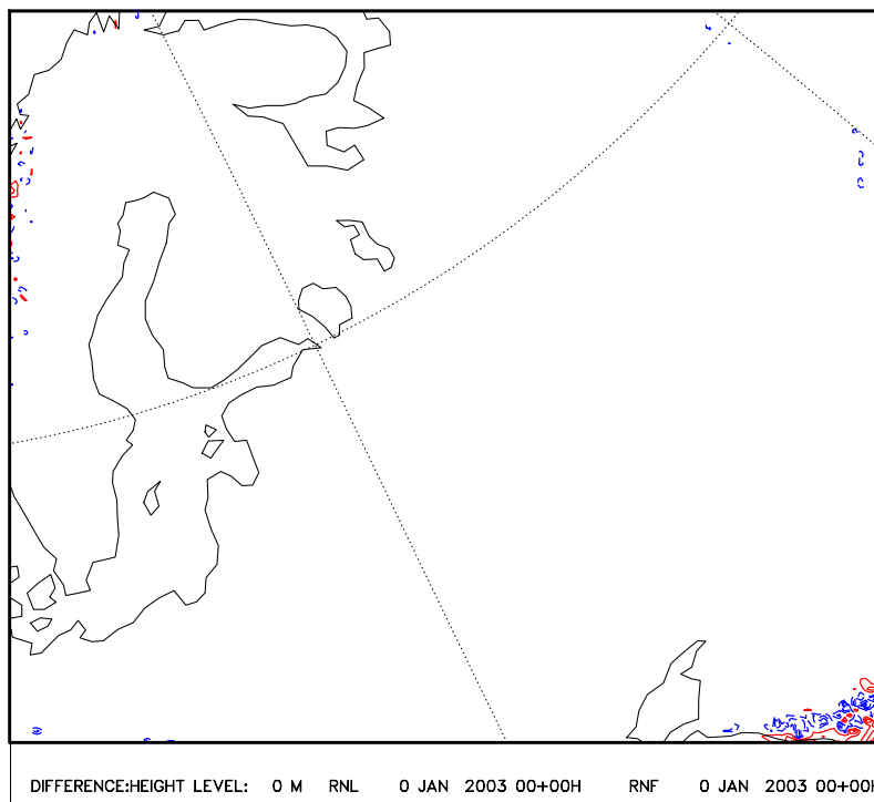
Figure 2: Difference between the relaxed (RNL) and the original (RNF) orography (RNL-RNF) for the nested system. Contour interval: 100 m. The zero isoline not plotted, negative values indicated with dashed lines.
