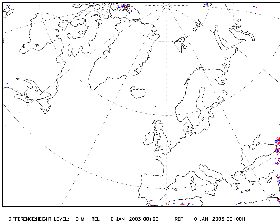
Figure 1: Difference between the relaxed (REL) and the original (REF) orography (REL-REF). Contour interval: 100 m. The zero isoline not plotted, negative values indicated with dashed lines.
