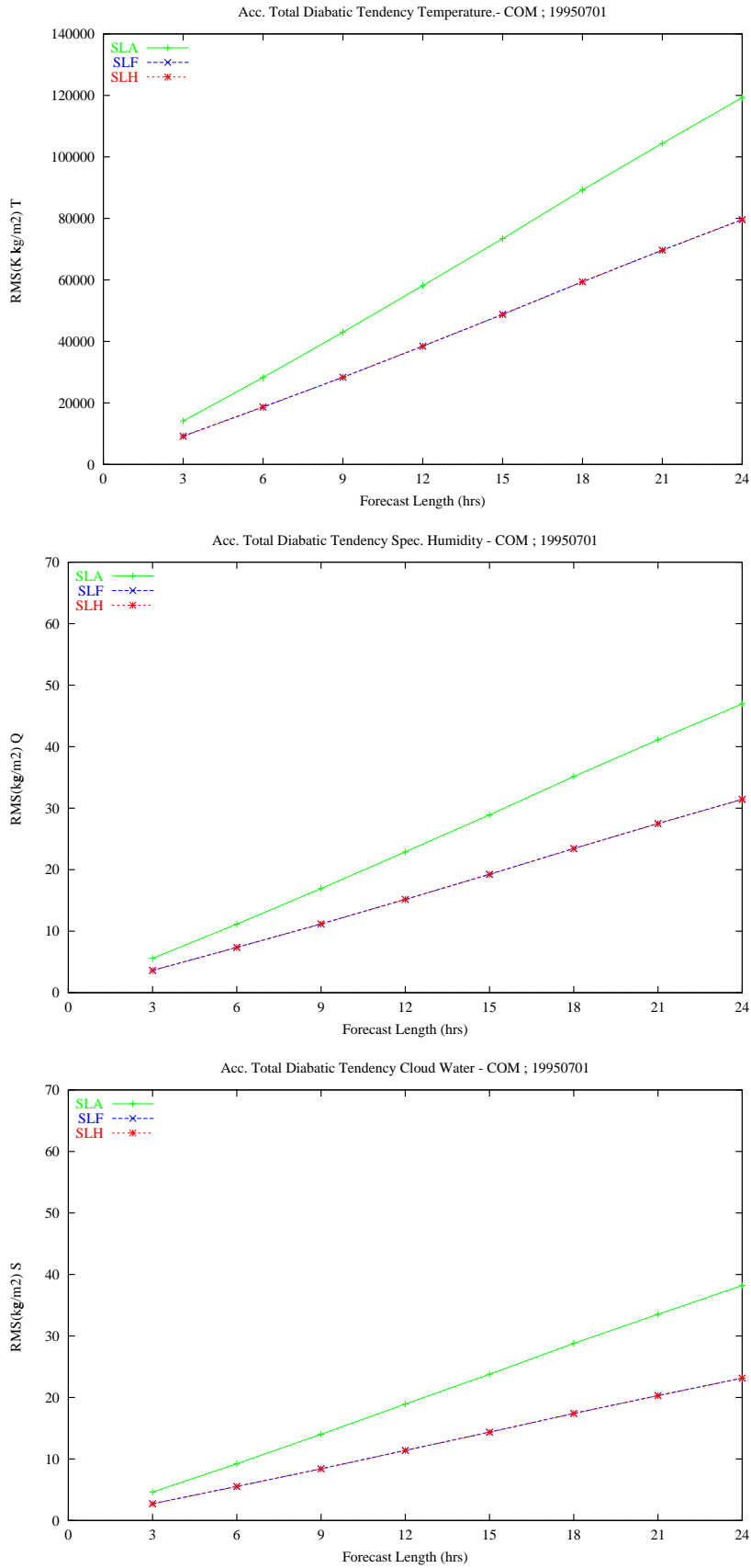
Figure 1: Root mean square error as described in equation (9) of the accumulated total diabatic tendencies of temperature ( top ), specific humidity ( center ) and cloud water content ( bottom ).
