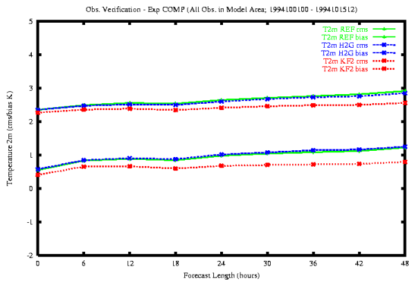
2 m Temperature
