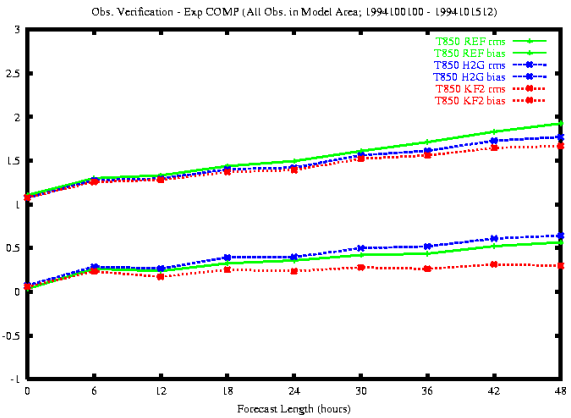
850 hPa Temperature
