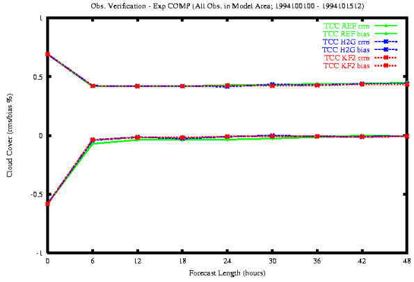
Total Cloudiness
