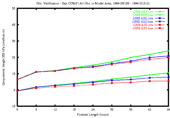
500 hPa Geopotential
